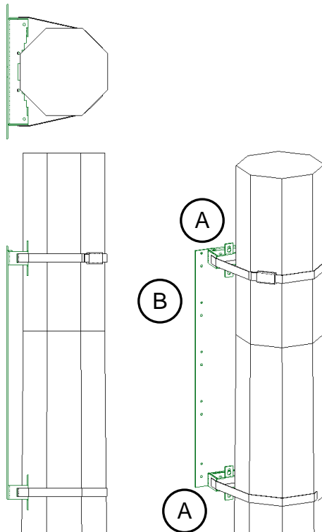
Figure 27 – Pole mounting example
