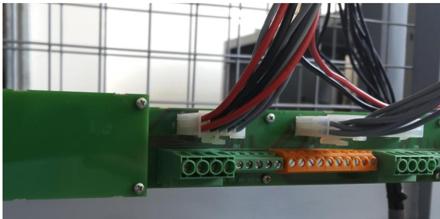
Figure 18 – Cables from SG and DFPI connection to the terminal board by means of Molex connector
