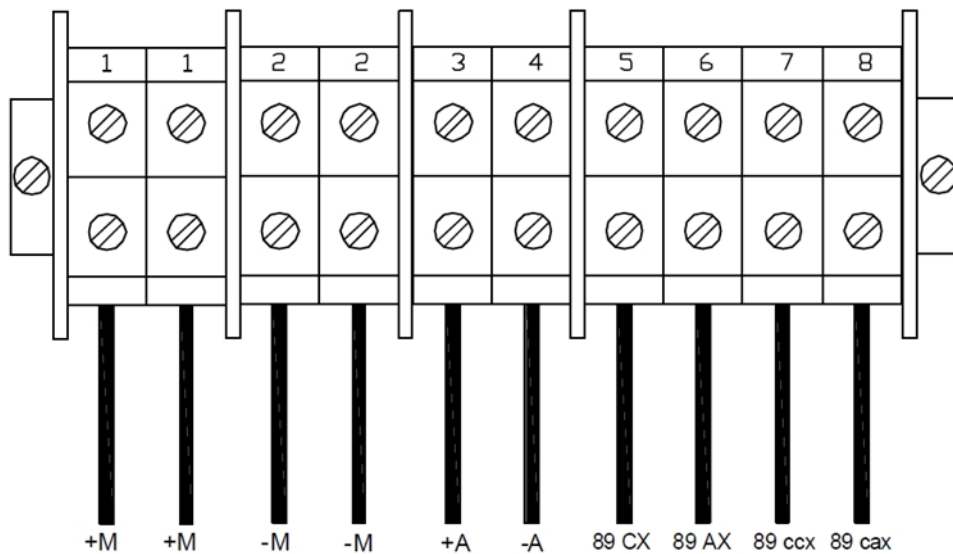
Figure 21 - Pre-wiring of the terminal board, in detail.
