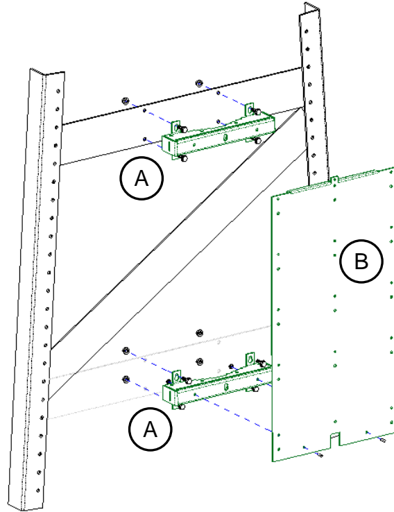
Figure 26- Pylon mounting example
