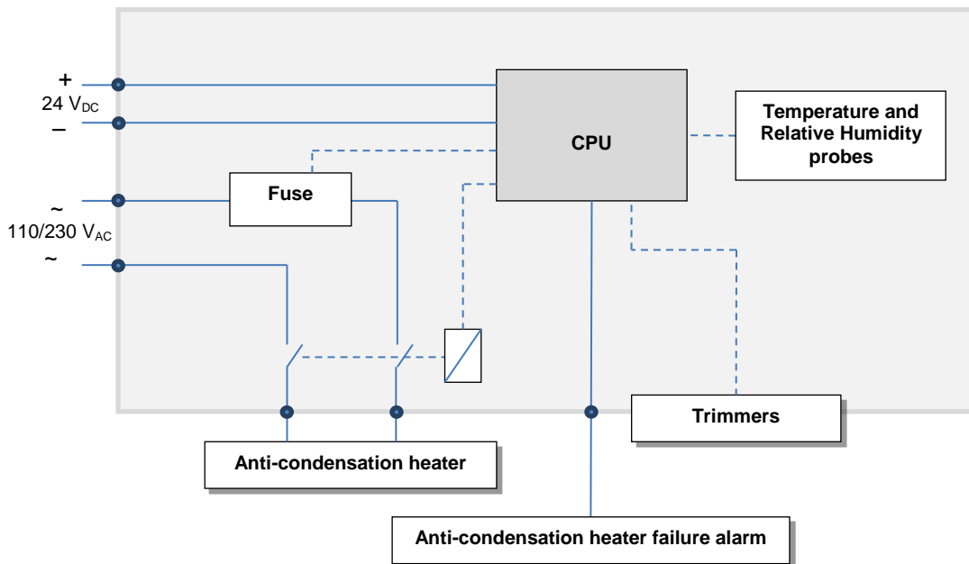
Figure 22 – Anti-condensation heater and temperature controller
