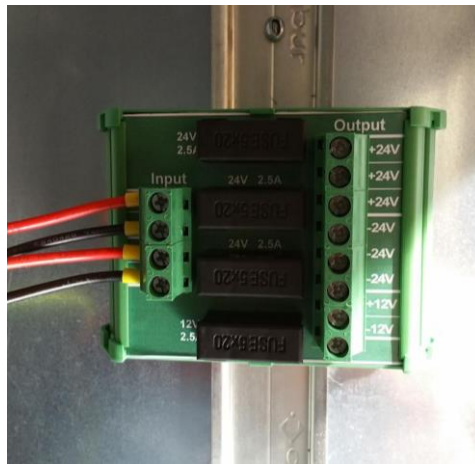
Figure 20 – Terminal board for the distribution of the auxiliary power supplies
