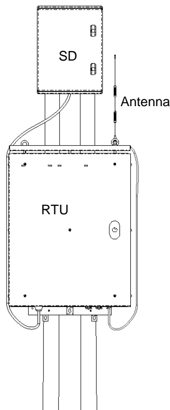
Figure 23 – Pole installation
