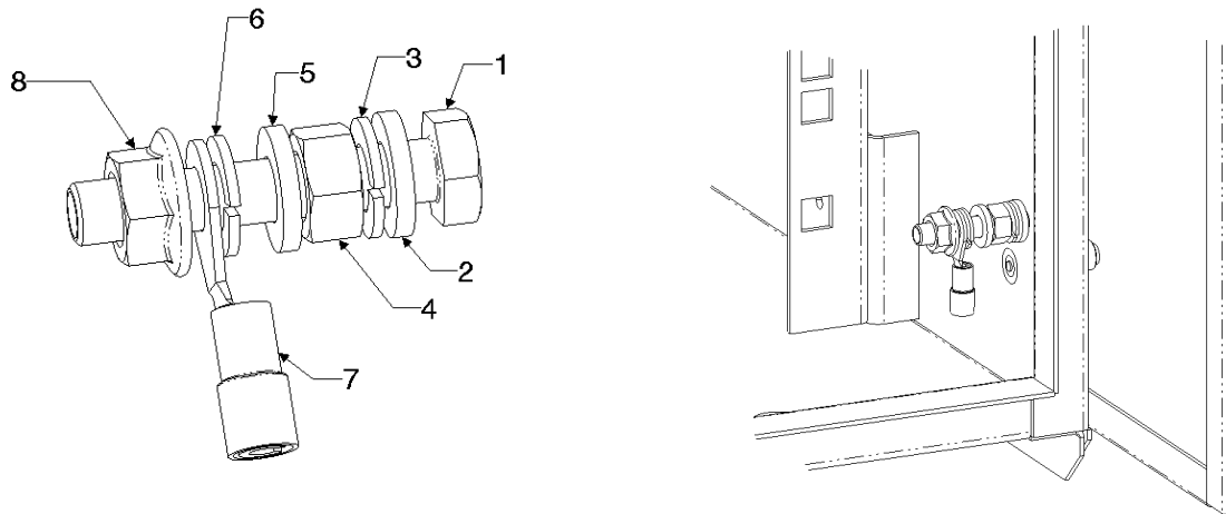
Figure 6 - Grounding bolt
