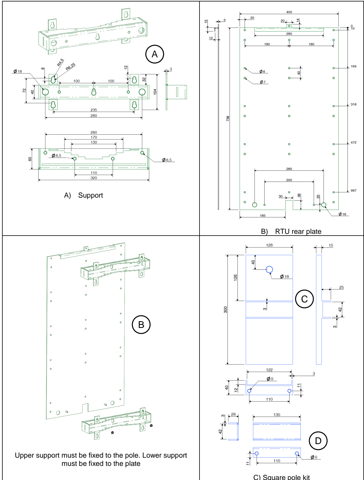
Figure 24 – RTU pole mounting kit
